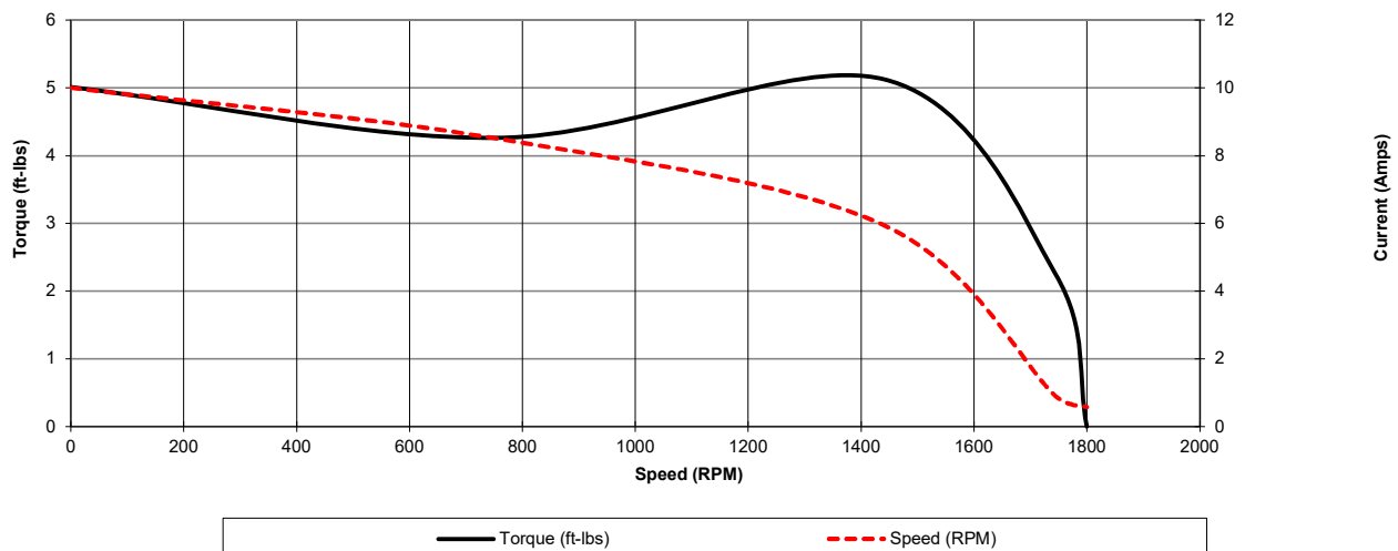
443T - 464T Dual Voltage SGL 3 Leads WYE Connection
